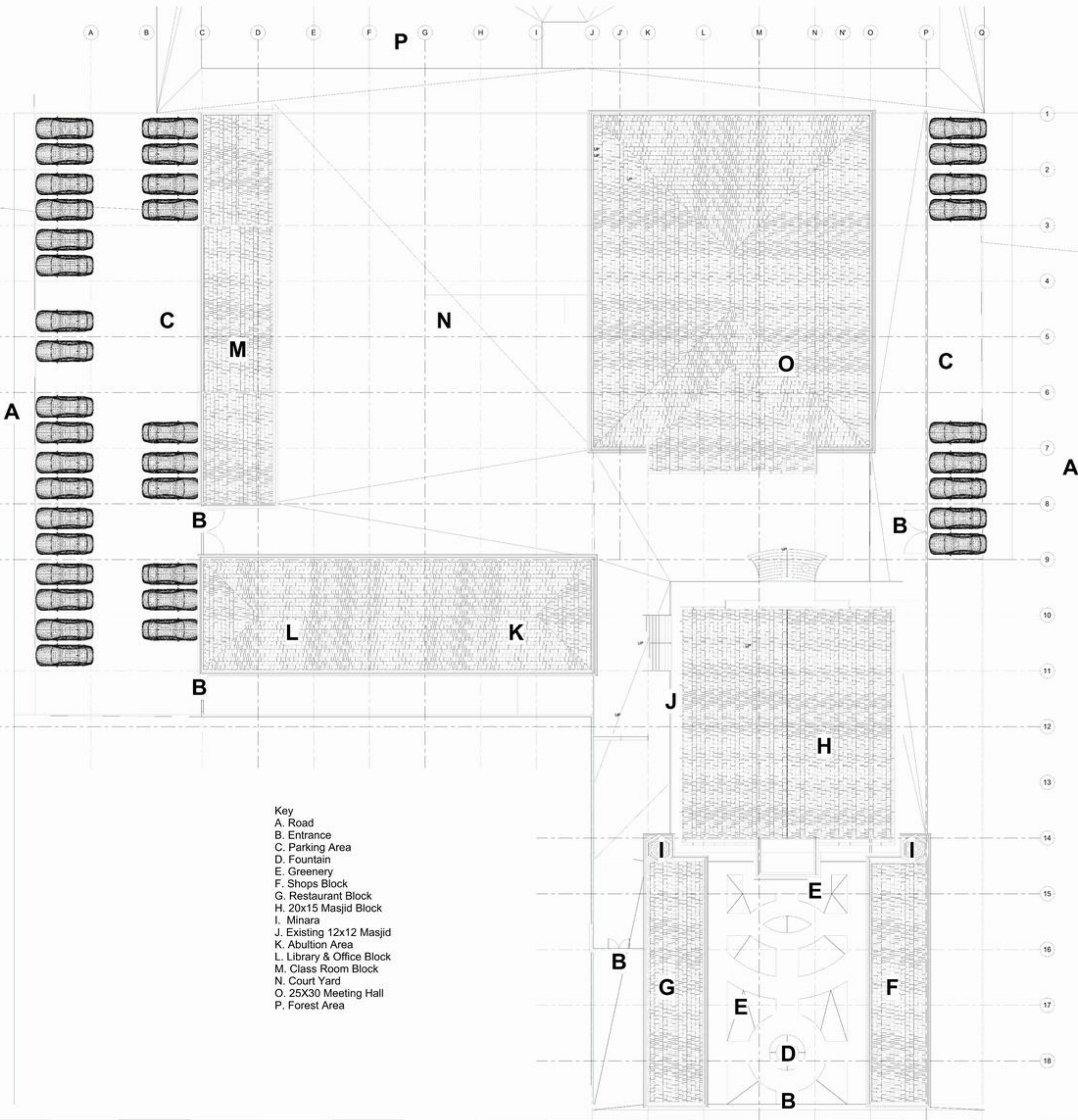
Site Plan
