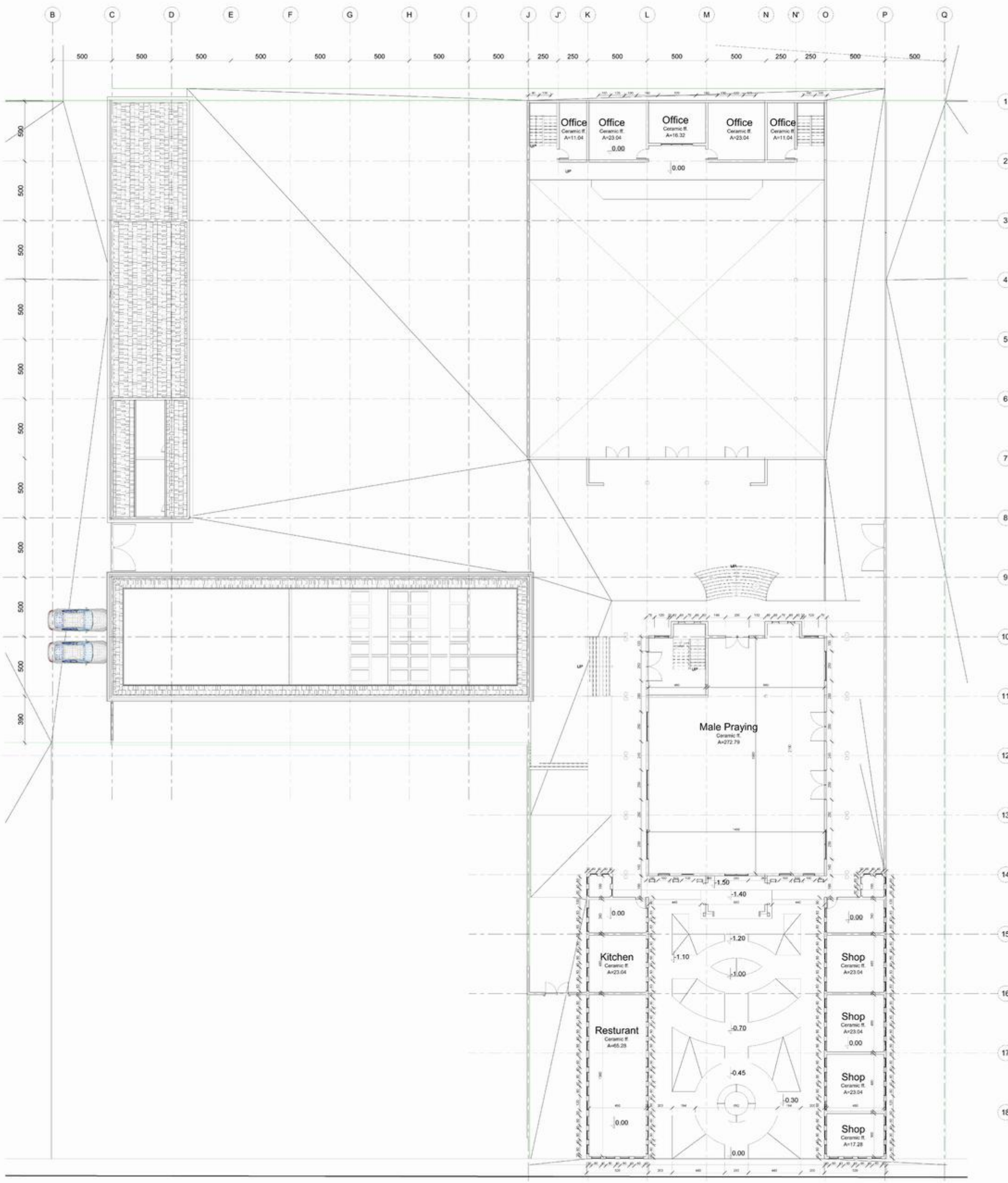
Floor Plan @-1.50
